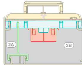
Wirefill #2: Power and Communication using Sloped Screw-on Communication Faceplate.
