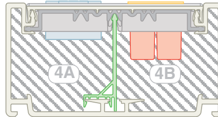
Wirefill #4: T130 Raceway — Power and data using T130RMC2 Faceplate.
