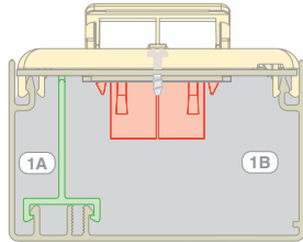
Wirefill #1: Power and Communication using Vertical Sloped Snap-on Communication Faceplate.
