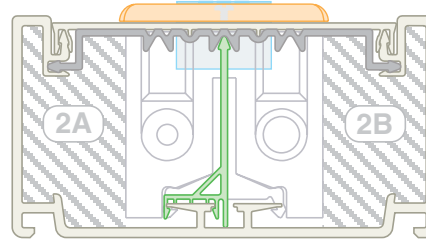
Wirefill #2: T130 Raceway — Power and data using T Box and U.S. Standard “Screw-on” Electrical/Communication Faceplates.
